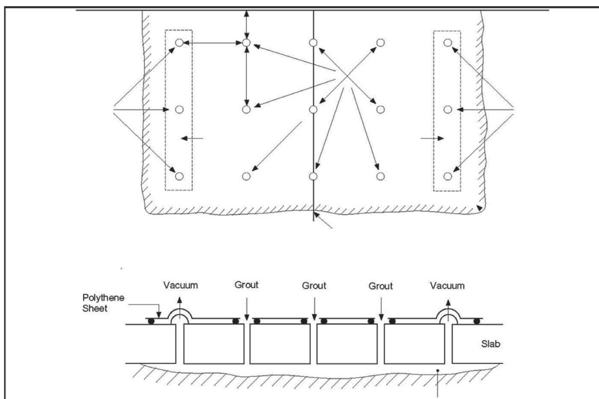
FIGURE 10/1: Vacuum Grouting Diagram
